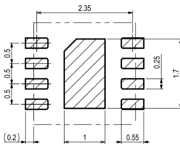
DFN8 (2.5*2.5)
