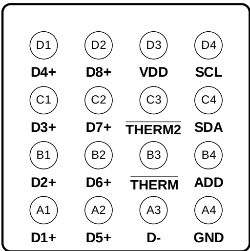
WLCSP-16 Top View
