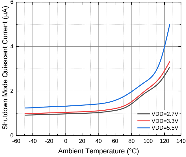
Quiescent Current in Shutdown Mode vs Ambient Temperature
