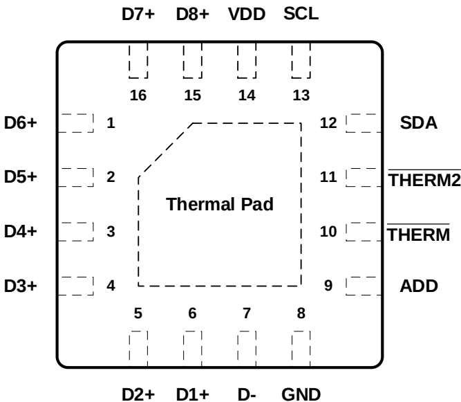
QFN-16 Top View
