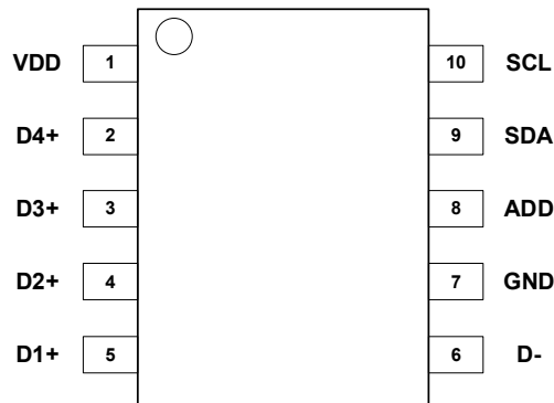
GXTR304 10-PIN MSOP Package
