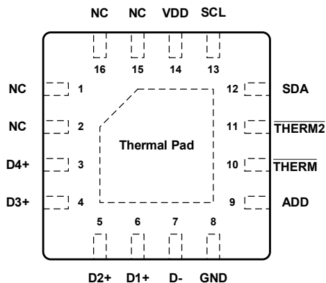
GXTR304 16-PIN VQFN Package
