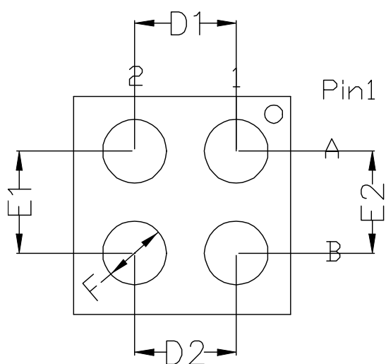
Bottom View(Ball up)
